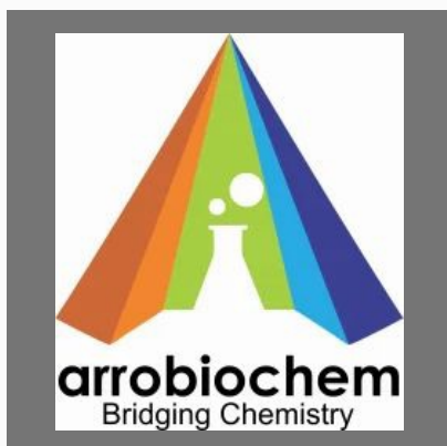
Potassium Chloride 99%
