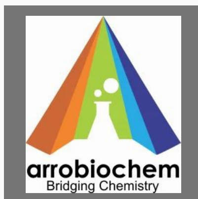
TRIETHYLAMINE HYDROCHLORIDE 98%
