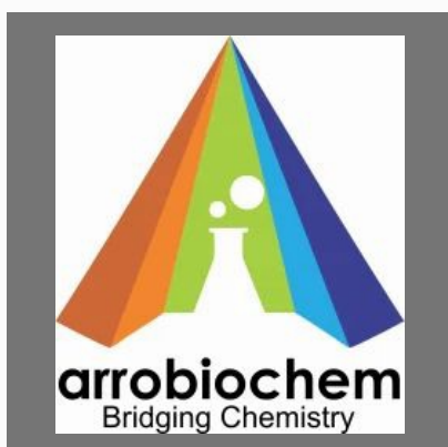
Trimethylacetyl Chloride, 98%
